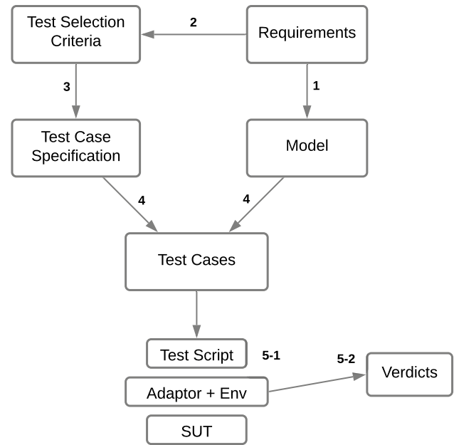
Fig. 1 MBT process diagram from Utting et al. [69]
